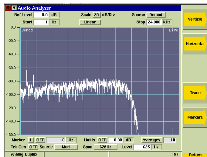
Figure 6. Audio Analyzer
