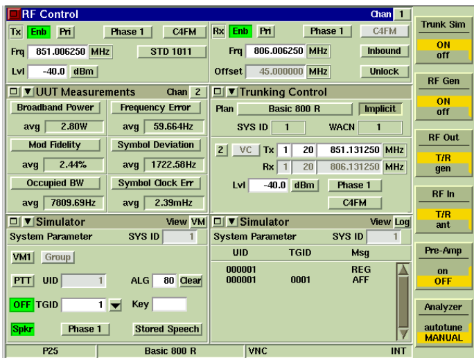
Figure 11. P25 Trunking Simulation
